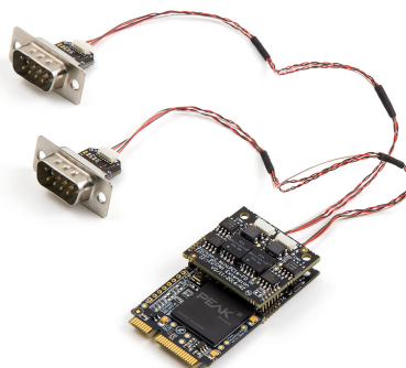
PCAN-miniPCle FD
